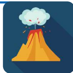
tectonic plates
